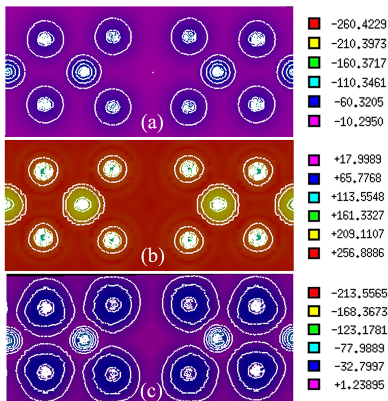
Figure 6 Contour plots for v_{x,\sigma}^{BR}(\vec{r}) and \sqrt{\frac{t_{\sigma}(\vec{r})}{\rho_{\sigma}(\vec{r})}} contributions of the total v_{x,\sigma}^{mBJ}(\vec{r}) exchange potential of \gamma\text{-Al}_2\text{O}_3 . Two-dimensional plots for (a) v_{x,\sigma}^{BR}(\vec{r}) and (b) \sqrt{\frac{t_{\sigma}(\vec{r})}{\rho_{\sigma}(\vec{r})}} contributions of (c) the total v_{x,\sigma}^{mBJ}(\vec{r}) exchange potential for \gamma\text{-Al}_2\text{O}_3 . v_{x,\sigma}^{BR}(\vec{r}) is obtained from Equation 3 by setting c = \frac{2}{3} , and \sqrt{\frac{t}{\rho}} is obtained from Equation 3 by setting c = 0 . v_{x,\sigma}^{mBJ}(\vec{r}) is obtained from Equation 3 using the optimized c -factor, i.e., c = 1.8 .
